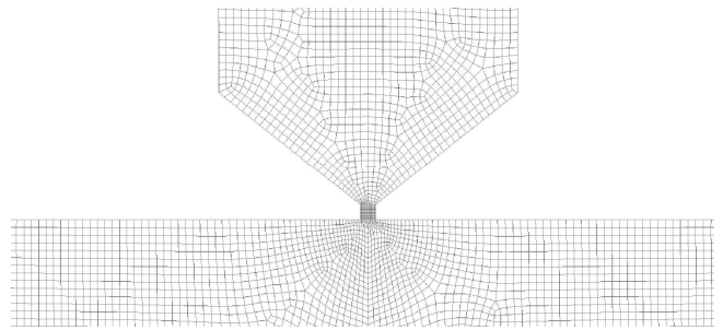
Fig. 13. View of the hexahedral mesh used in analysis, in a plane through the centerline of the model
