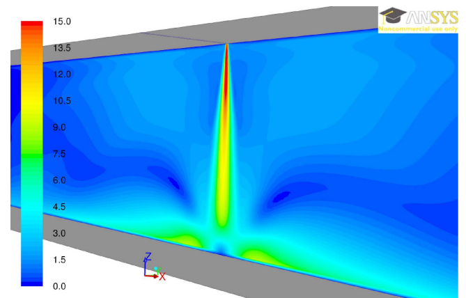
Fig. 6. Contours of velocity (0–15 m/s), for U_o = 27 m/s, I = 0.5\% , \alpha = 0^\circ , realizable k-\epsilon turbulence model [5]
