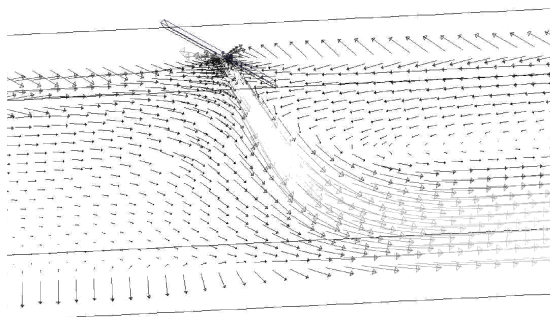
Fig. 17. Velocity vectors at the proximity of air curtain (0–5 m/s) for U_o = 10 m/s, I = 0.5\% , \alpha = 30^\circ , HRR = 6.0 MW, fire on the right side of air curtain
