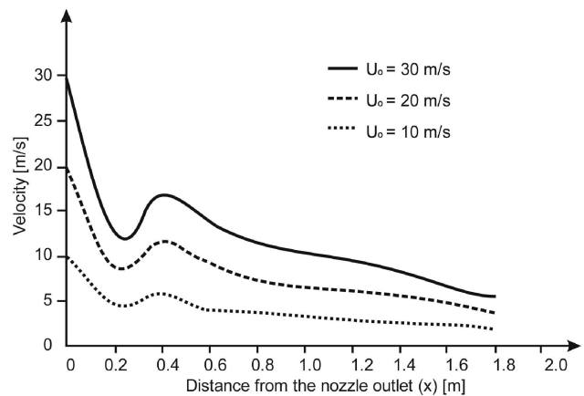
Fig. 10. Velocity of the air in the distance from the nozzle outlet in x axis for different U_o values (Ref. 19)
