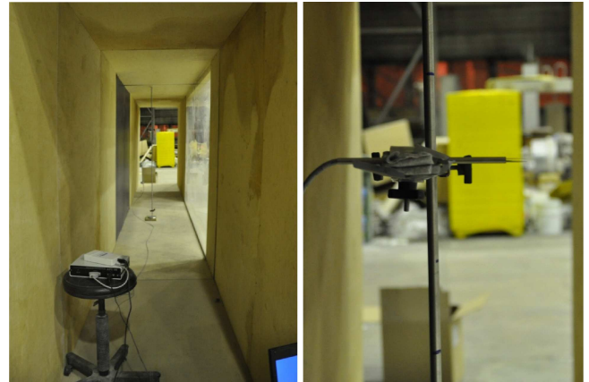
Fig. 9. Interior (left) and measuring equipment of the test tunnel (Ref. 19)
