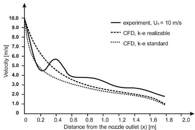
Fig. 11. Velocity of the air in the distance from the nozzle outlet in x axis from experiment and CFD studies (Ref. 19)
