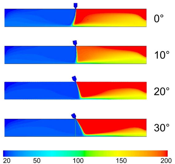
Fig. 20. Temperature plot (20–200°C), for U_o = 30 m/s, I = 0.5\% , \Delta p = 10 Pa, \alpha = 0^\circ, 10^\circ, 20^\circ and 30^\circ
