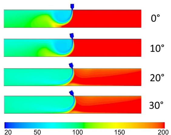
Fig. 14. Temperature plot, for U_o = 10 m/s, I = 0.5\% , \Delta p = 6 Pa, \alpha = 0^\circ, 10^\circ, 20^\circ and 30^\circ
