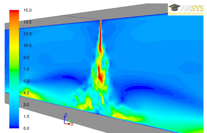
Fig. 7. Contours of velocity (0–15 m/s), for U_o = 27 m/s, I = 0.5\% , \alpha = 0^\circ , LES turbulence model (Ref. 5)
