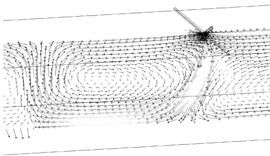
Fig. 18. Velocity vectors at the proximity of air curtain (0–5 m/s) for U_o = 10 m/s, I = 0.5\% , \alpha = 30^\circ , HRR = 13.0 MW, fire on the right side of air curtain
