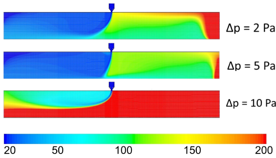
Fig. 15. Temperature plot, for U_o = 10 m/s, I = 0.5\% , \Delta p = 3.5 and 10 Pa, \alpha = 0^\circ
