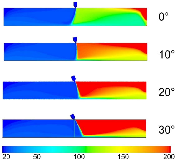
Fig. 19. Temperature plot (20–200°C), for U_o = 20 m/s, I = 0.5\% , \Delta p = 10 Pa, \alpha = 0^\circ, 10^\circ, 20^\circ and 30^\circ
