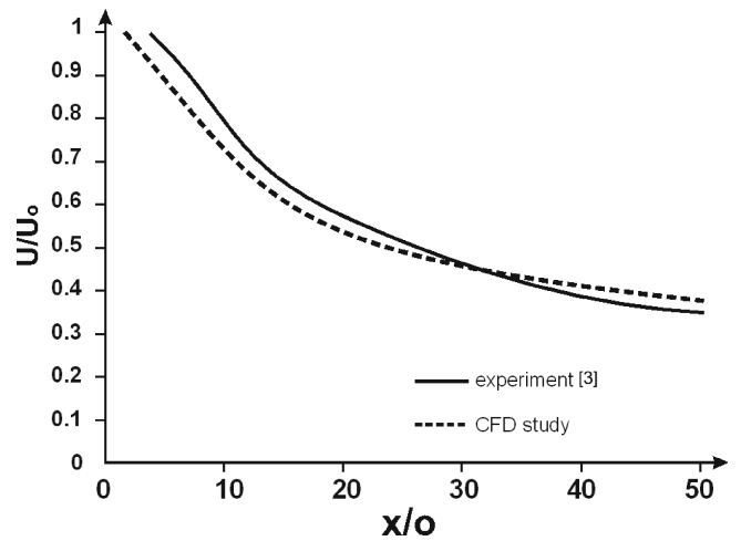
Fig. 5. Results of centreline velocity decay, for U_o = 27 m/s, I = 0.5\% , \alpha = 0^\circ [5]
