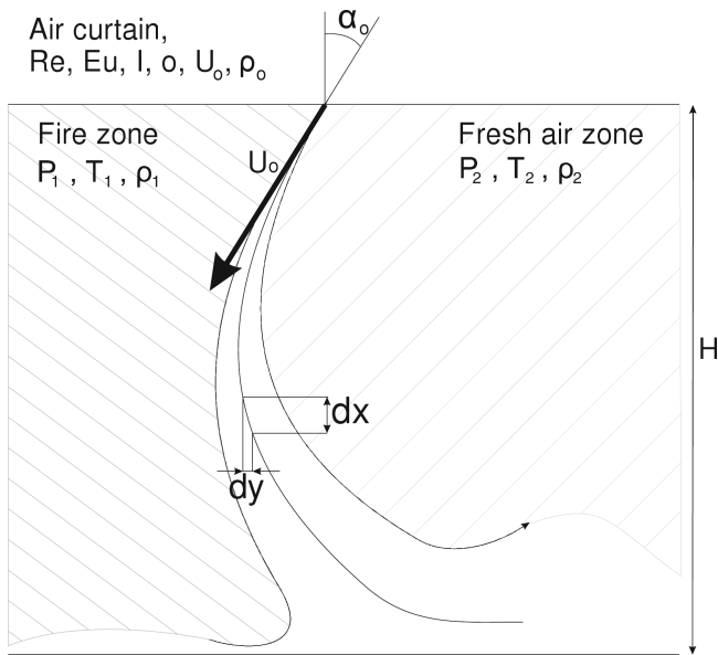
Fig. 4. Air curtain with air induced at angle \alpha , with visual presentation of variables that influence the flow (own work, based on Ref. 11)
