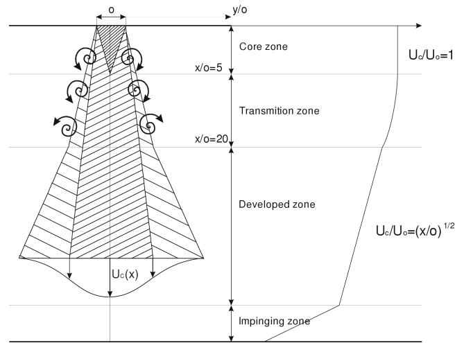
Fig. 3. Regions of air curtain, left side of figure presents possible shape of the air curtain, right side shows change of U_c/U_o along symmetry plane of curtain in x dimension (own work, based on Ref. 6)
