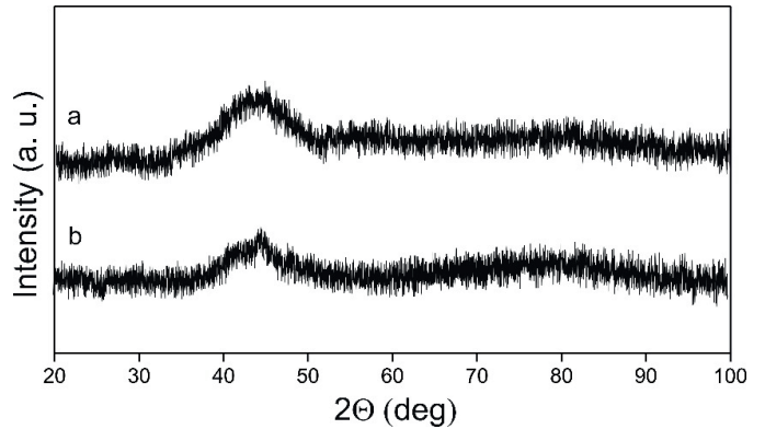
Fig. 1. X-ray diffraction patterns for the investigated alloys of Fe_{63}Co_{10}Y_7B_{20} (a) and Fe_{64}Co_{10}Y_6B_{20} (b), in the as-quenched state
