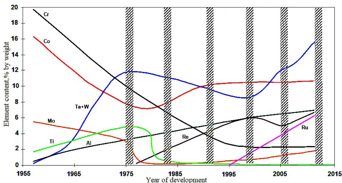
Fig. 1. Dependence of changes in the chemical composition of superalloys on the year of development
