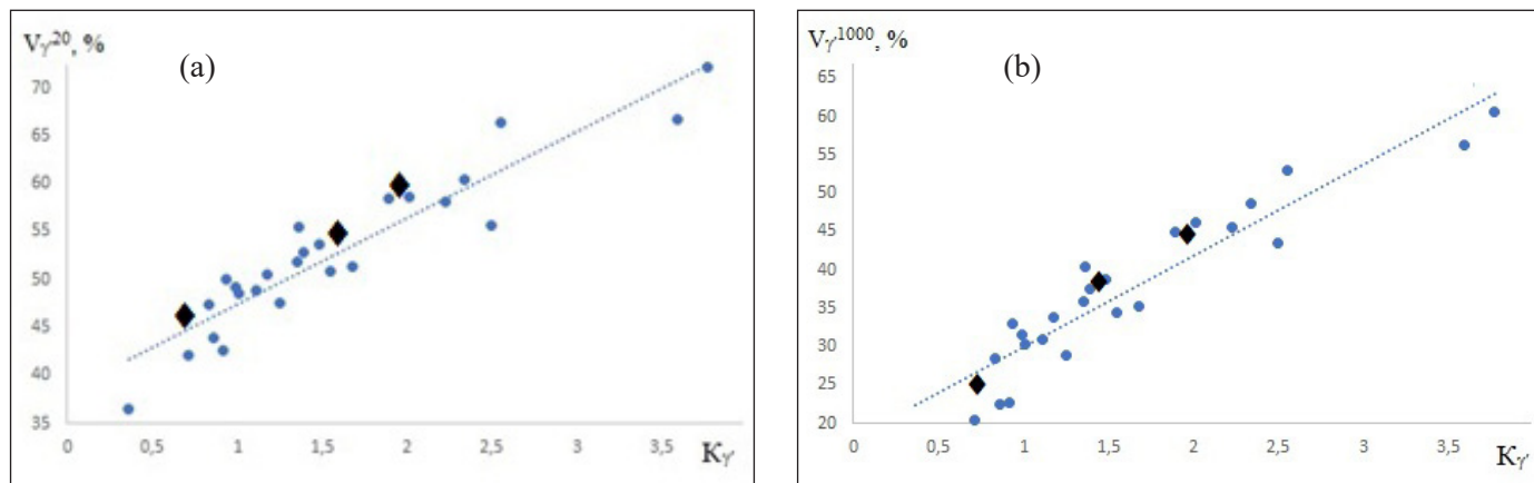
Fig. 4. Correlation dependences of the volume of the \gamma' -phase in equiaxed superalloys on the ratio of K\gamma' in their composition (a) – dependence of the volume of the фазы-phase at room temperature ( V_{\gamma'20} , %) on the value of the ratio K\gamma' ; (b) – dependence of the volume of the \gamma' -phase at 1000°C ( V_{\gamma'1000} , %) on the value of the ratio K\gamma' (● – calculated values; ♦ – experimental values)
