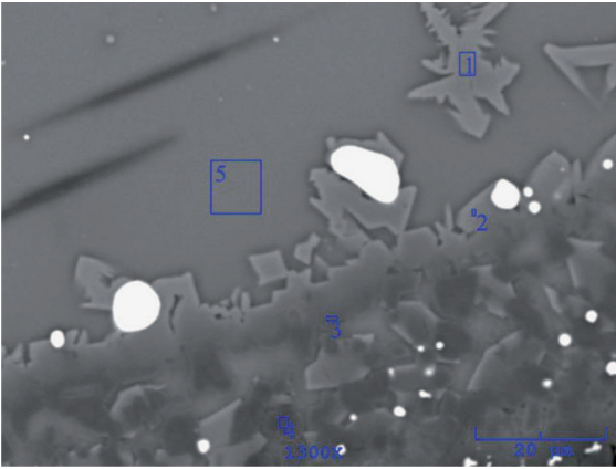
Fig. 7. Tundish cover slag with grains of well blocking sand
