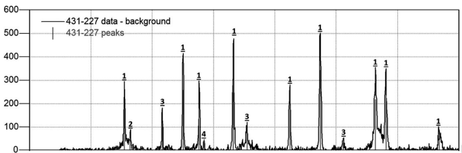
Fig. 2. XRD diagram of cover powder, phases marked with: 1- Al 2 O 3 , 2- SiO 2 , 3-C, 4-Al
