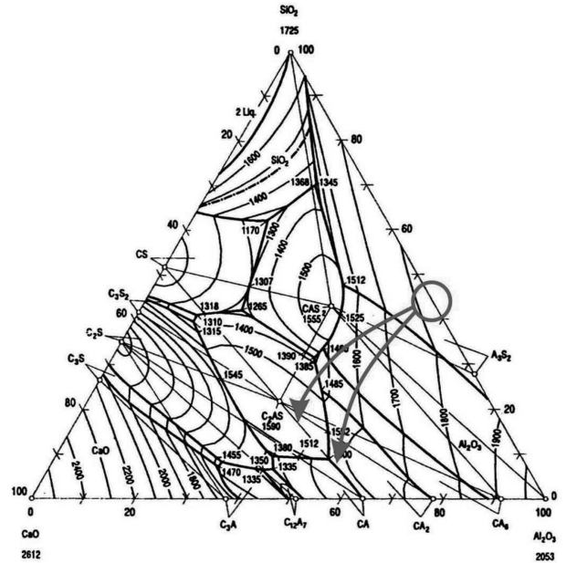
Fig. 14. Ternary phase diagram Al_2O_3 \cdot CaO \cdot SiO_2 [7]
