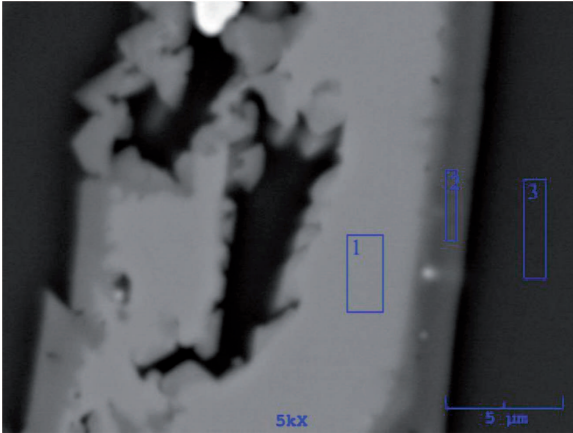
Fig. 8. Chromite grain with MnO enriched border area
