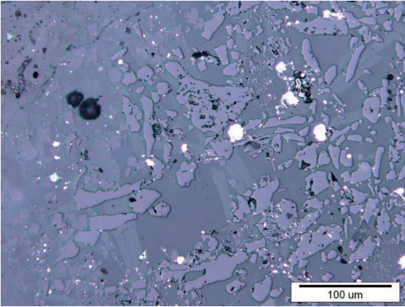
Fig. 9. Microstructure of a melted cover slag
