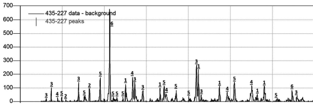
Fig. 11. Cover slag deposits on thermocouple protective shroud. 1: Al_2O_3 , 2: SiO_2 , 3: 2CaO \cdot Al_2O_3 \cdot SiO_2 , 4: MgO \cdot Al_2O_3 , 5: CaO \cdot 2Al_2O_3 , 6: CaS
