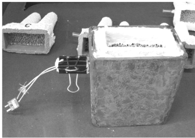
Fig. 1. Mould prepared for an experiment
