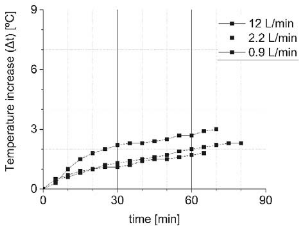
Fig. 9. Temperature increase diagram for bearing with elastic polymer bush. Test conditions: pressure=0.4 MPa, shaft revolution speed =10 rev/s, water flow=0.9-12 L/min.
