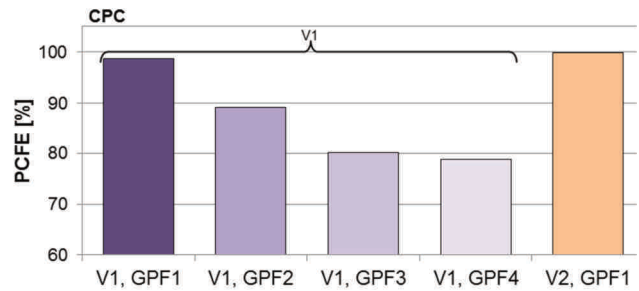
Fig. 10. PCFE's of the investigated GPF's in WLTC hot
