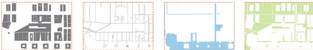
Fig. 4. Almere - Noorderplasen. List of spatial structure elements: Analyzed area: 127,5 ha. Built-up areas: 46.9 ha - 37%, Communication: 10.6 ha - 8%, Water: 27 ha - 21%, Greenery: 43 ha - 34%. Source: autor
