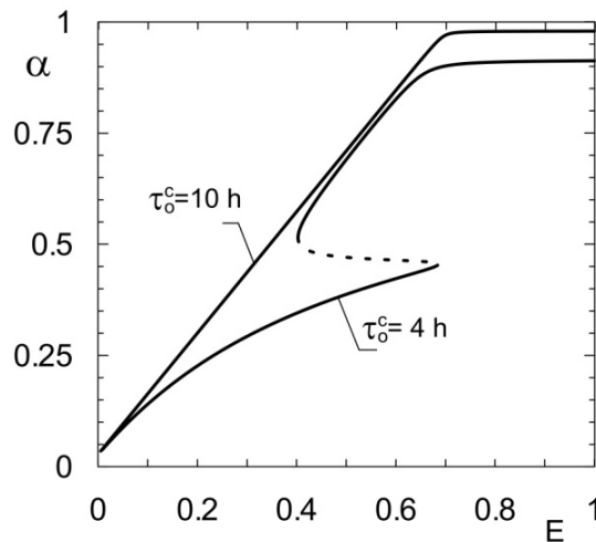
Fig. 6. Effect of external aerator efficiency E on a degree of conversion of carbonaceous substrate ( c_{Af} = 0.2 \text{ kg/m}^3 ; L_b = 3 \cdot 10^{-5} \text{ m} ; \vartheta = 0 ; \xi = 0.98 ; \zeta_s = 0.01 )
