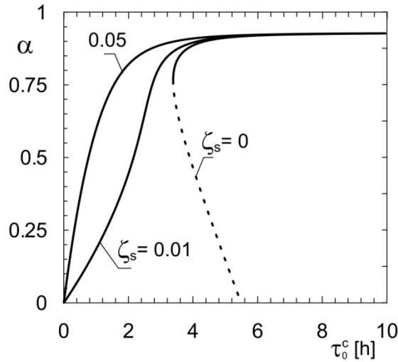
Fig. 5. Effect of the fraction of biofilm carriers in the liquid phase \zeta_s on the degree of conversion of carbonaceous substrate ( c_{Af} = 0.2 \text{ kg/m}^3 ; L_b = 3 \cdot 10^{-5} \text{ m} ; \vartheta = 0 ; \xi = 0.97 )
