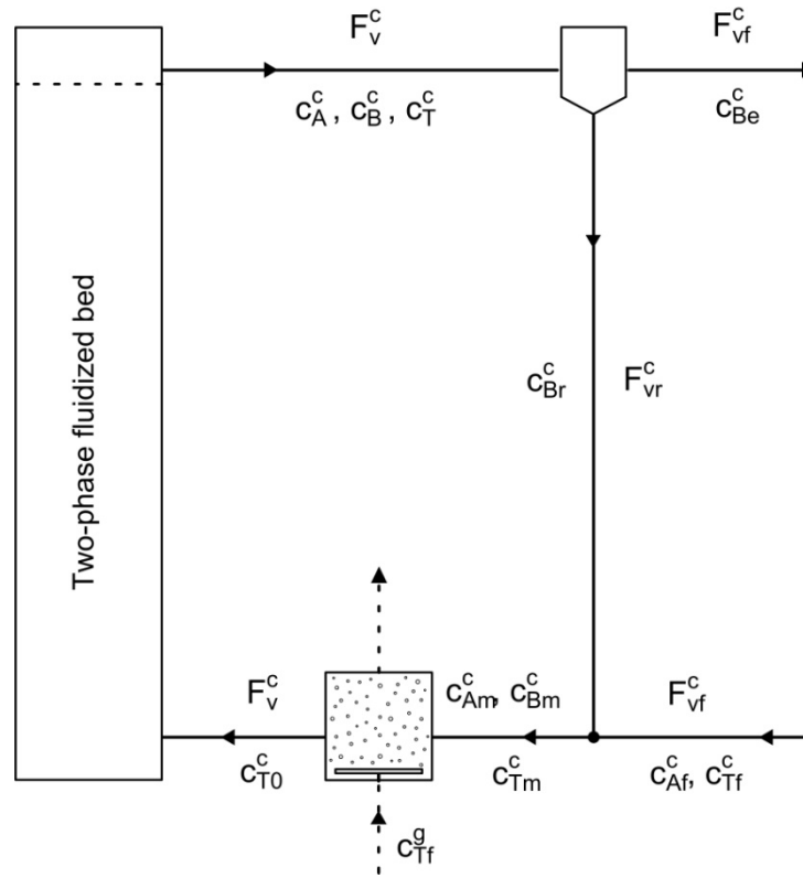
Fig. 1. Scheme of a two-phase fluidised bed bioreactor with an external aerator in the liquid recycle loop
