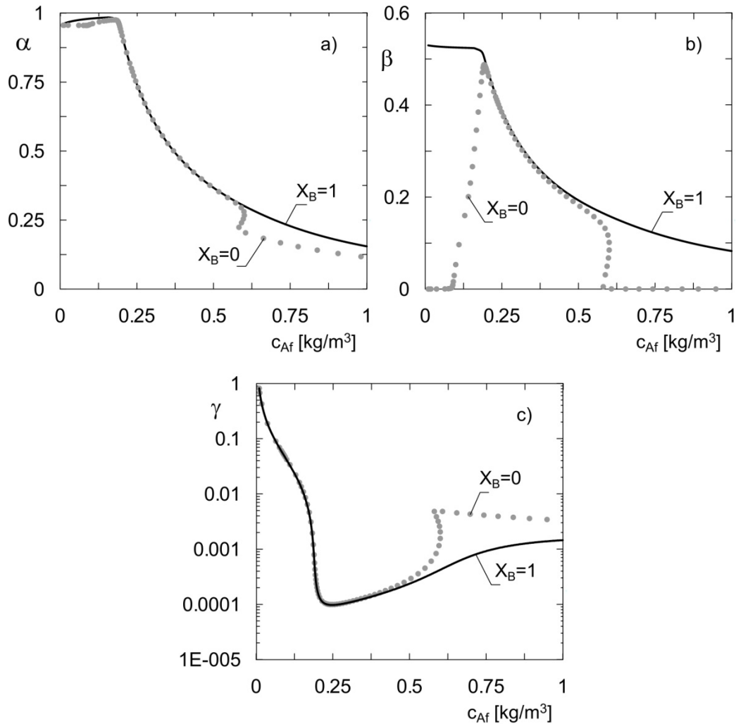
Fig. 4. Steady state branches \alpha(c_{Af}) , \beta(c_{Af}) and \gamma(c_{Af}) of a two-phase loop fluidised-bed bioreactor ( \tau_0^c = 10 \text{ h} ; L_b = 3 \cdot 10^{-5} \text{ m} ; \vartheta = 0 ; \xi = 0.97 ; \zeta_s = 0.01 )
