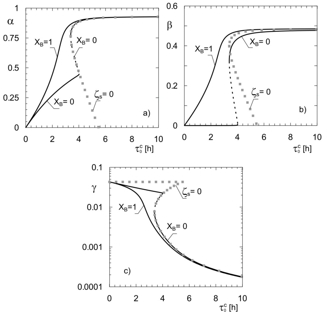
Fig. 3. Stationary properties of a two-phase loop fluidised-bed bioreactor ( c_{Af} = 0.2 \text{ kg/m}^3 ; L_b = 3 \cdot 10^{-5} \text{ m} ; \vartheta = 0 ; \xi = 0.97 ; \zeta_s = 0.01 ) — stable steady states; - - - - - unstable steady states
