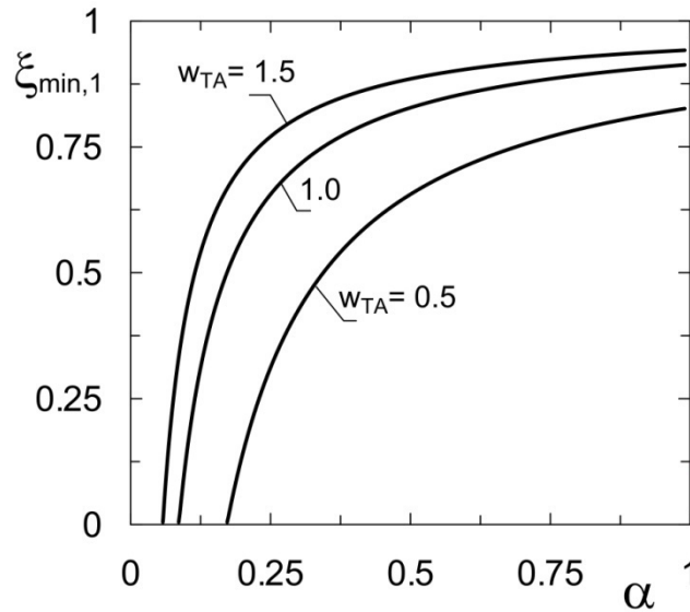
Fig. 2. Dependency of \xi_{min,1} on the degree of conversion of carbonaceous substrate \alpha and the yield coefficient w_{TA} ( c_T^* = 0.0086 \text{ kg/m}^3 ; c_{Af} = 0.1 \text{ kg/m}^3 )
