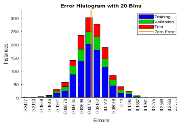
Figure 8. Error histograms obtained during the learning process for the fastest analyzed neural network
