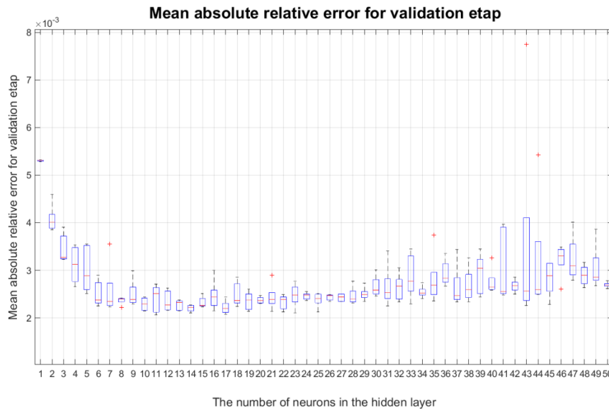
Figure 4. Mean absolute relative error obtained for the obtained for the neural network structure with a certain number of neurons in a hidden layer
