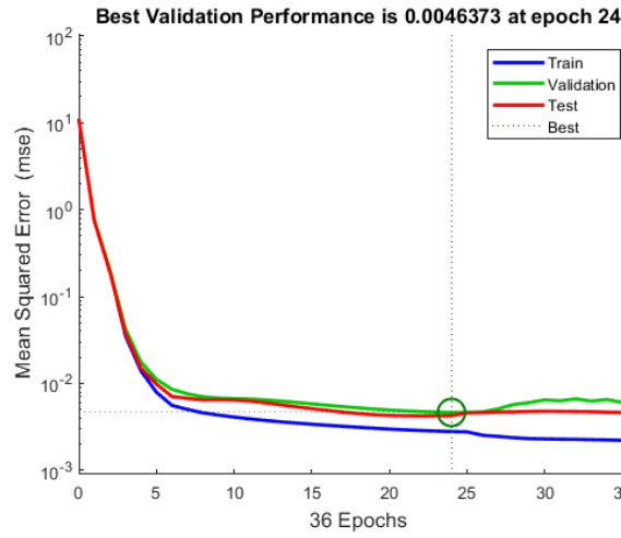
Figure 6. Performance function values obtained during the learning process for the fastest analyzed neural network
