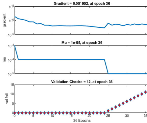
Figure 7. Gradient, momentum, and validation checks values obtained during the learning process for the fastest analyzed neural network
