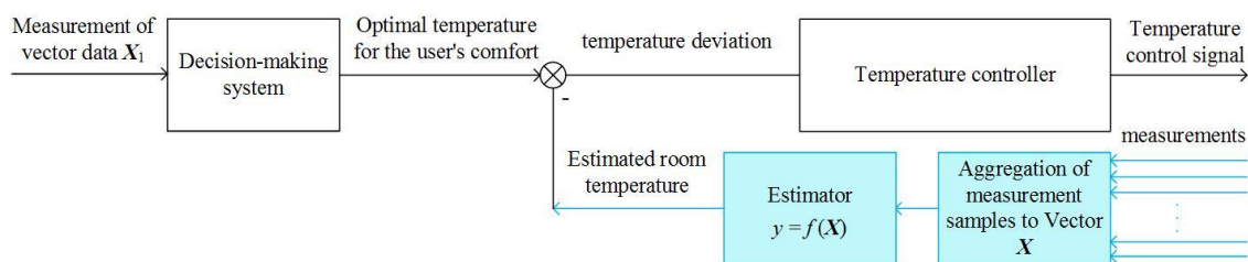
Figure 1. Partial schematic use in the building control system
