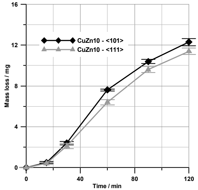
Fig. 10. Average mass loss vs. exposition time plots obtained for CuZn10 alloy tested on the jet-impact stand
