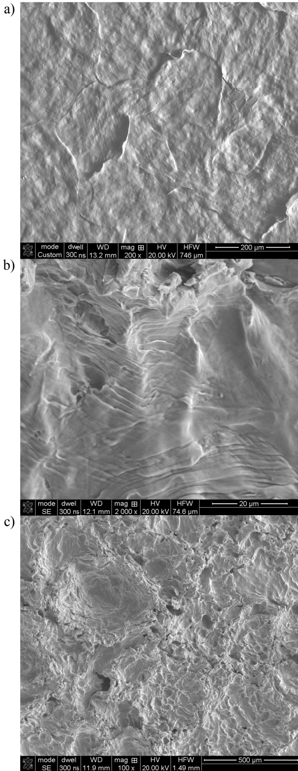
Fig. 9. The state of the CuZn10 <101> // ND alloy surface after test on the jet impact stand: a) the uplifting of grain boundaries zones after 5 min, b) shear bands located in near grain boundaries areas after 15 min, c) cavities and craters on the sample surface after 90 min
