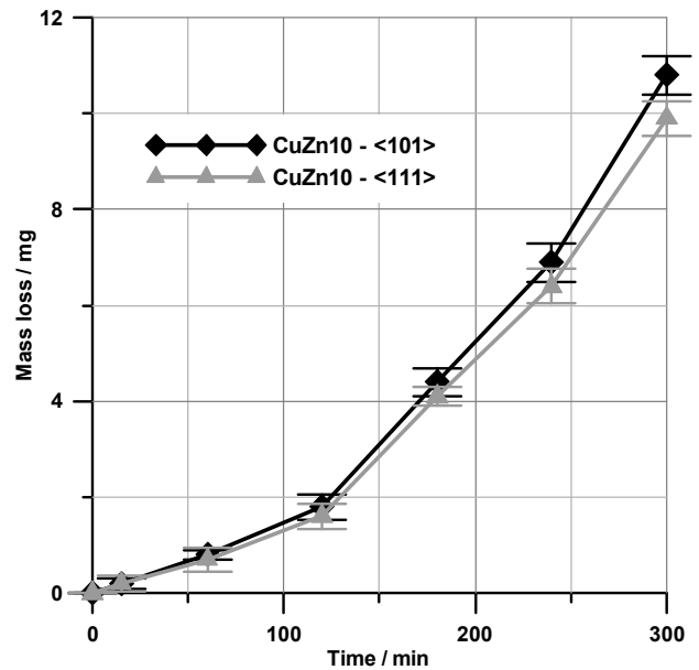
Fig. 11. Average mass loss vs. exposition time plots obtained for samples CuZn10 alloy tested on the flow stand
