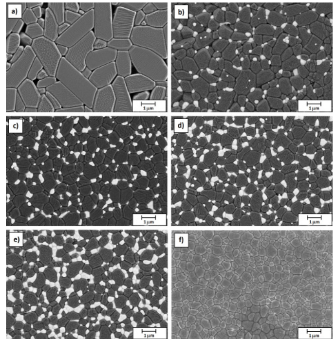
Fig. 4. SEM images of sintered bodies; in ceramic suspensions ACR-MAN was used as the monomer
