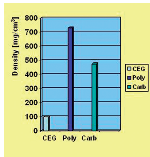
Fig. 5. Apparent density changes of compressed expanded graphite (CEG) after impregnation with furfuryl alcohol, polymerization (POLY) and subsequent carbonization to 550^\circ\text{C} (CARB). The initial density of CEG was 100 \text{ mg/cm}^3
