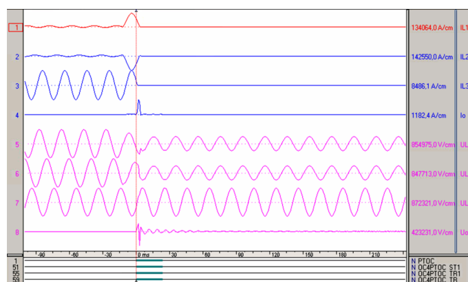
Fig. 9. Disturbance recording obtained during the testing of ABB REL670 over current function
