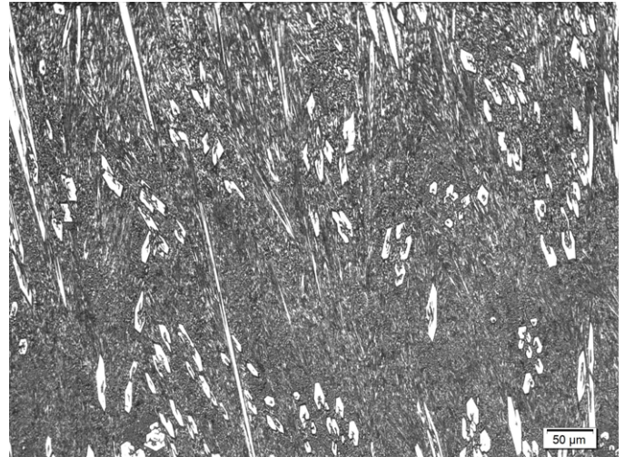
Fig. 3. Microstructure of sample B
