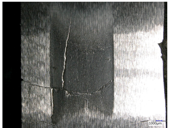
Fig. 9. The surface of the sample A after wear test
