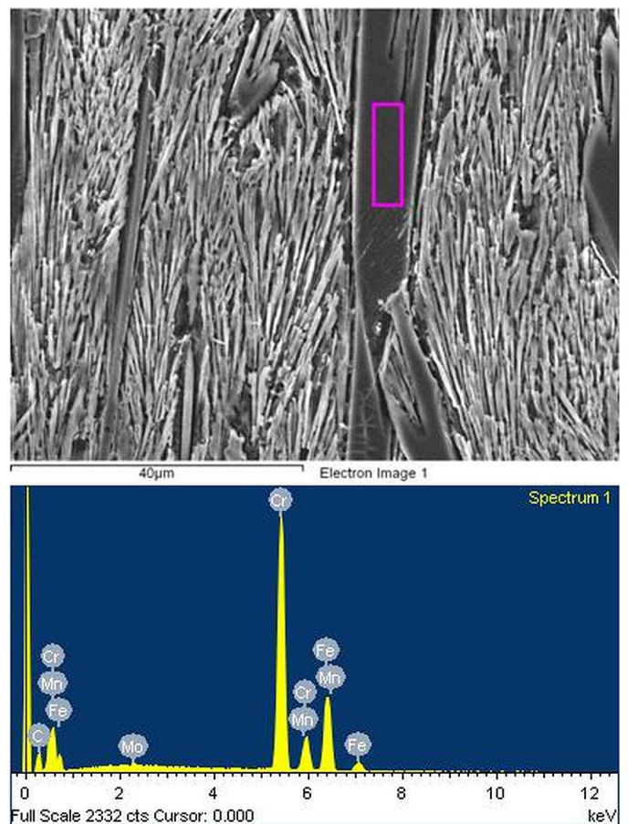
Fig. 4. SEM structure of sample B with chromium carbides
