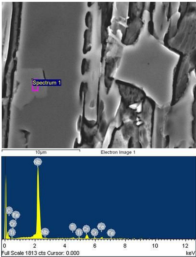
Fig. 2. SEM structure of sample A with Nb carbide inside chromium carbide
