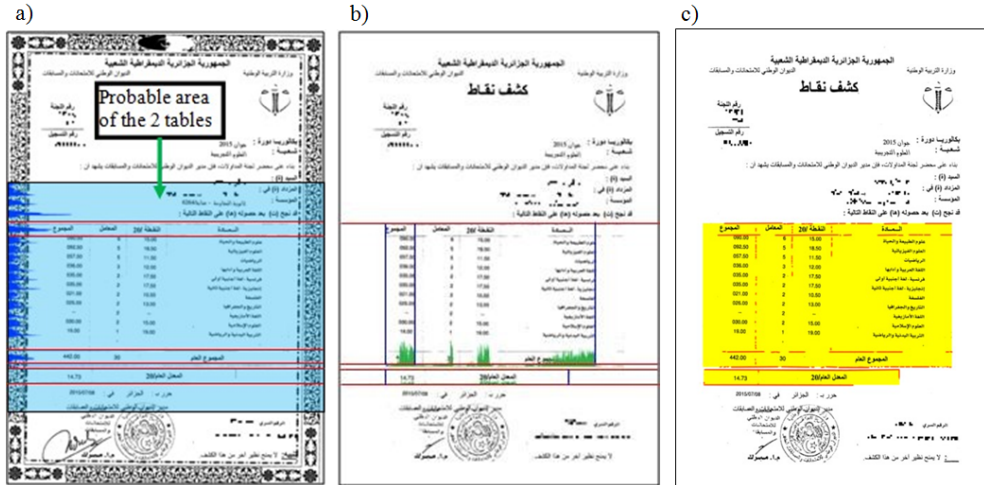
Figure 8. Localization of two tables: a) horizontal projection histogram of area containing two tables; b) vertical projection histogram and extraction of vertical lines; c) tables detected
