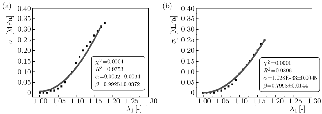
Fig. 4. Stress-strain curves described by new constitutive equation (3.6) for samples excised from walls of tested blood vessels: (a) AAA_c ; (b) AAA_l
