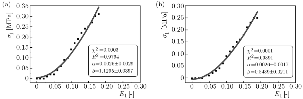
Fig. 3. Stress-stretch ratio curves described by constitutive equation (3.4) for samples excised from walls of tested blood vessels: (a) AAA_c ; (b) AAA_l
