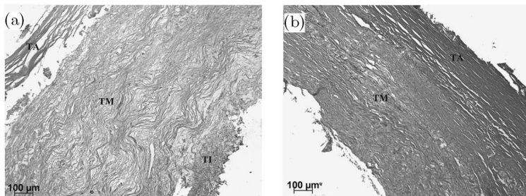
Fig. 2. Histological images of AAA walls: (a) with degenerated inner layer (TA – adventitia, TM – media, TI – intima), using H&E staining and (b) with atrophy of the inner layer, using Van Gieson’s staining
