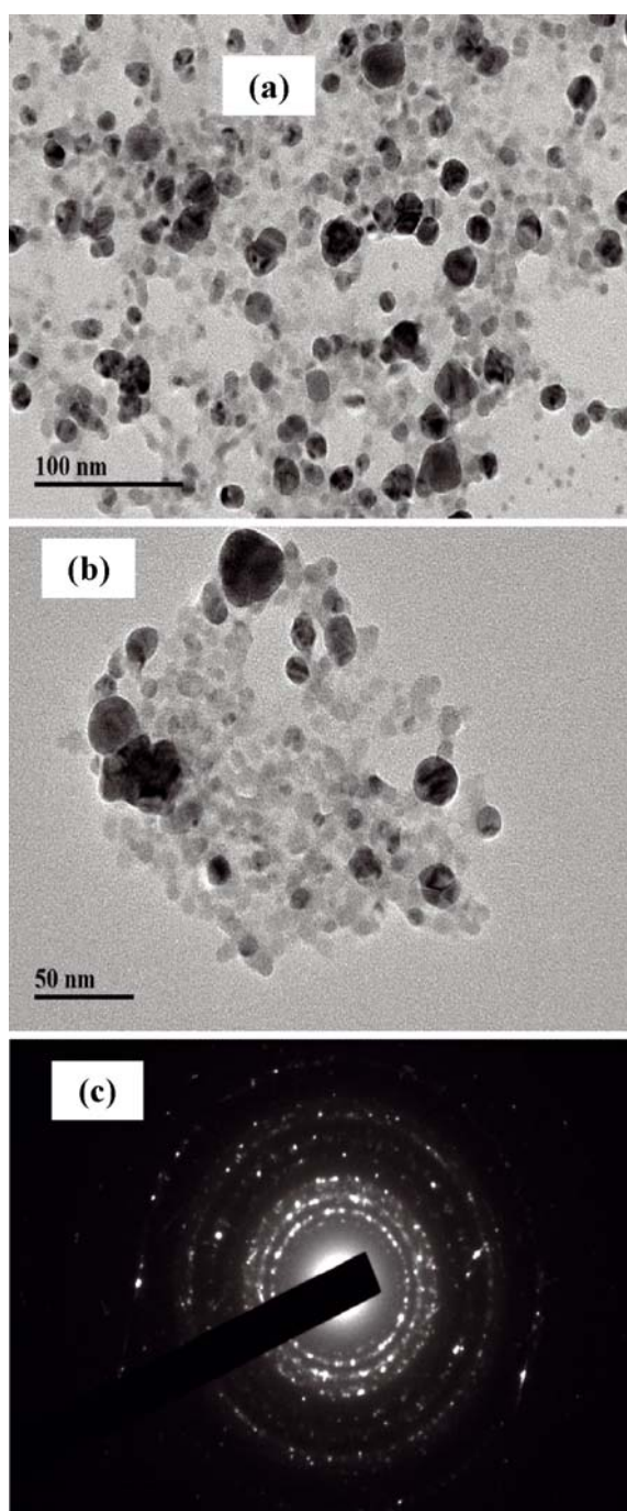
Figure 7. TEM micrographs for AgNPs using 0.01 M \text{AgNO}_3 solution at (a) 100 nm, (b) 50 nm magnifications and (c) SAED patterns of AgNPs
