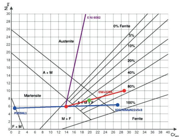
Fig. 1 The Schaeffler's diagram [17]
