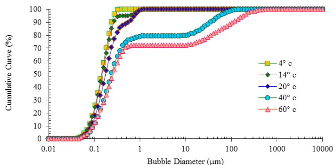
Fig. 15. Influence of temperature on bubble size distribution
