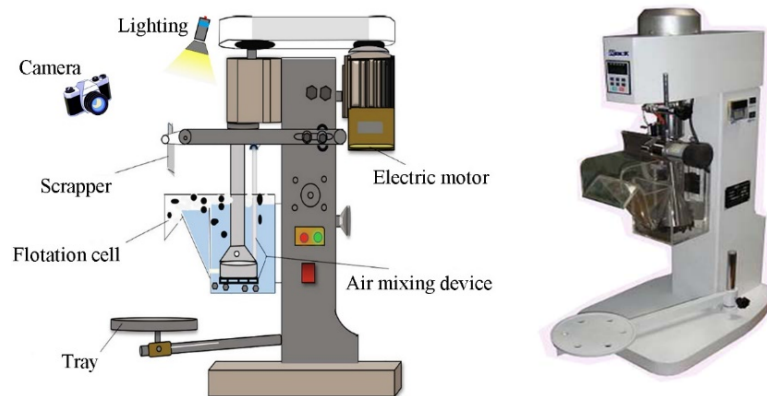
Fig. 1. Experimental set-up for the flotation experiments (left: schematic diagram, right: physical photo). Adapted from the literature (Zhou et al., 2020; Bu et al., 2018)
