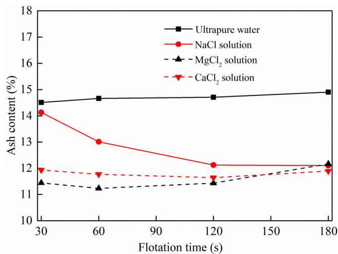
Fig. 5. The ash content of clean coal obtained in ultrapure water, NaCl, MgCl 2 , and CaCl 2 solutions
