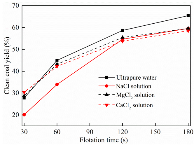
Fig. 4. The clean coal yield of ultrapure water, NaCl, MgCl 2 , and CaCl 2 solutions
