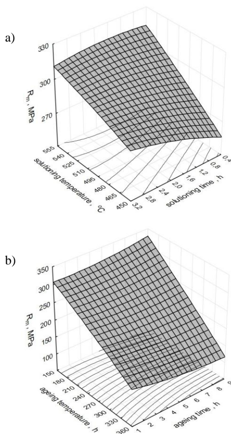
Fig. 5. Change of the R_m strength of the AlSi7Mg alloy in function of time and temperature a) solutioning, b) ageing
