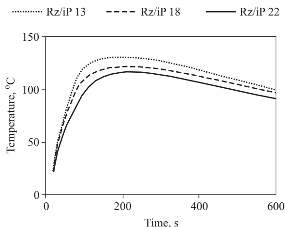
Fig. 1. Temperature profiles of core of foams synthesized using the bio-polyol from rapeseed oil (Rz) and isopropanol (iP) (Rz/iP 13; Rz/iP 18; Rz/iP 22 – symbols of foam with 13, 18 and 22 wt % of the bio-polyol Rz/iP in polyol premix, respectively, according to [6])
