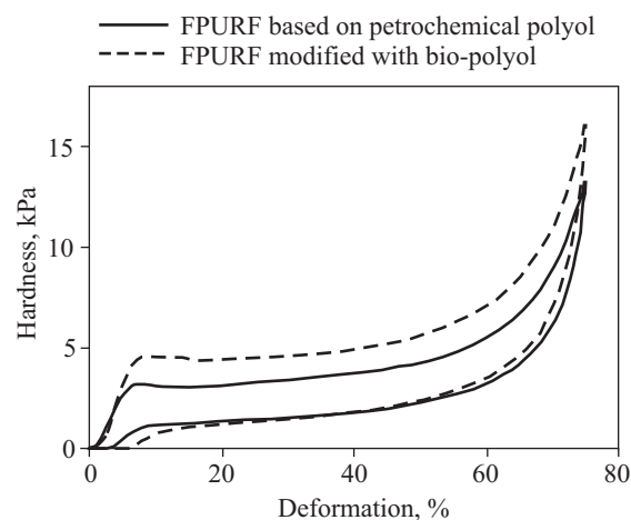
Fig. 2. Hysteresis loops of PUR foams (according to [70])
