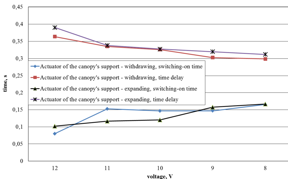
Fig. 7. Tests results for sliding down and up the canopy support’s actuator
