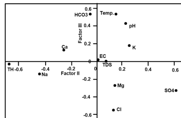
Fig.10. Plot of Factor II against Factor III
