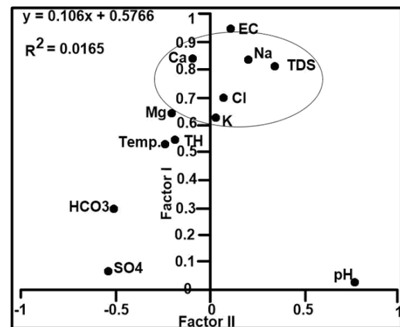
Fig.9. Plot of Factor I against Factor II.
