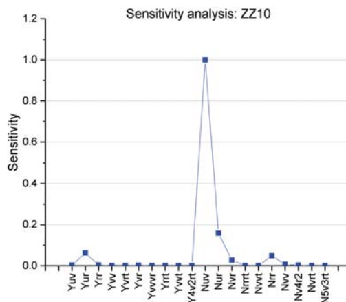
Fig. 4. Sensitivity analysis for zigzag manoeuvre
