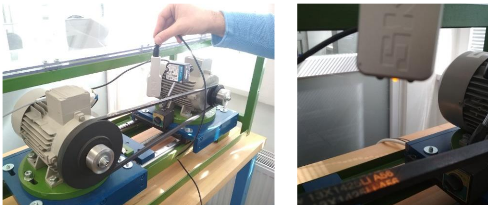
Fig. 5. Adjustment and tightening of the belt by means of contactless belt tension meter SKF
