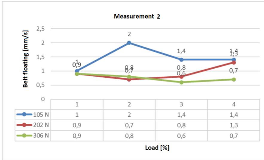
Fig. 7. Dependence of the belt floating on gear loading and the belt tightening at 1000 rev/min
