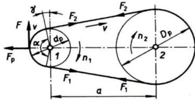
Fig. 1. Force ratio in the belt gear
