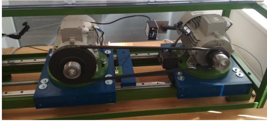
Fig. 3. Measuring system designed for the belt gear testing
