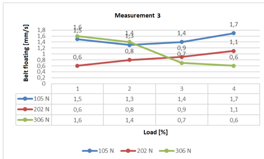
Fig. 8. Dependence of the belt floating on gear loading and the belt tightening at 1500 rev/min
