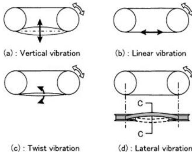
Fig. 2. Types of the belt floating
