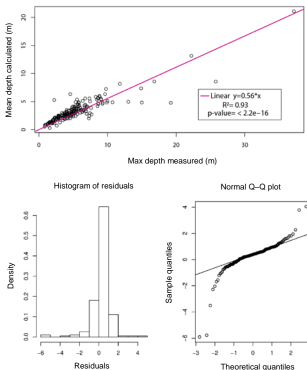
Fig. 10. Relationship between maximum measured depth and calculated average depth by dividing the query estimated volume and area of the lake polygon; source: own study
