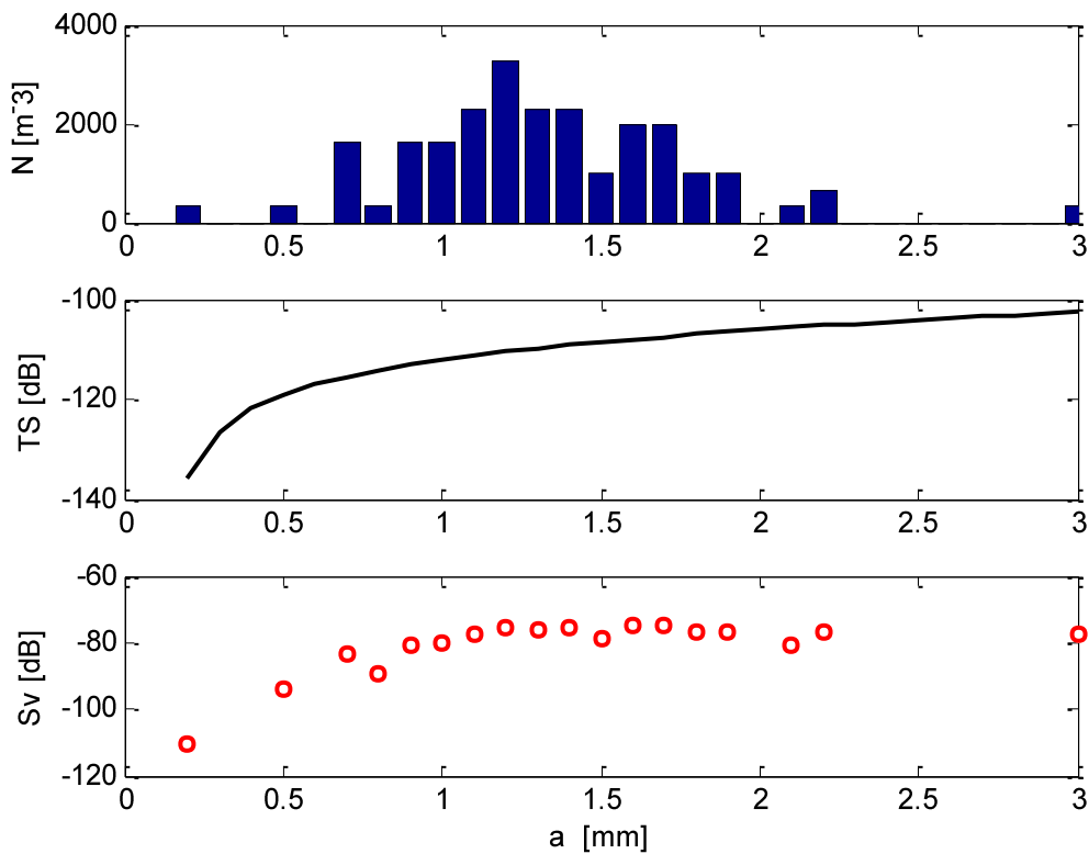
Fig.1. Histogram of plankton radii (upper), target strength calculated by model (middle) and contributions of particular size group to total backscattering (lower). Density contrast g=1 , sound speed contrast h=1.027 .
