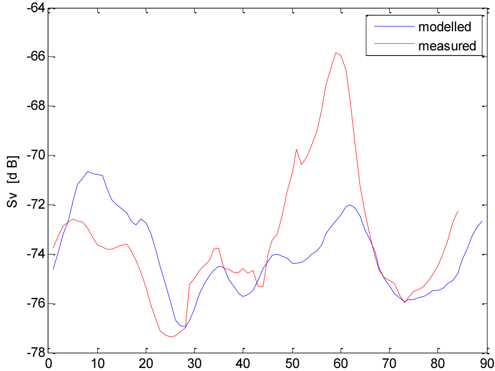
Fig.2. 47-minute echosounder record of S_v , measured by echosounder (red curve) and S_v , calculated by the model on the basis of zooplankton concentration measured by LOPC (blue curve) along the same transect at the same depth. Both signals are averaged over 60 transmissions (0.5 min). 31 July 2009.
