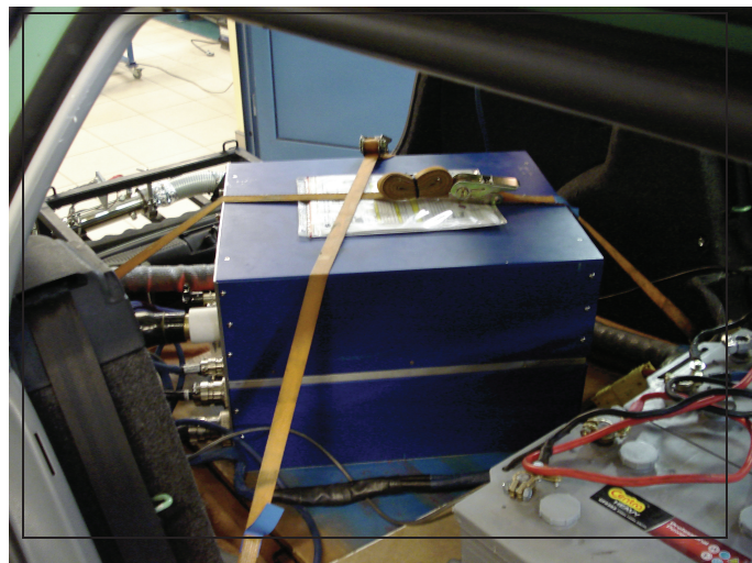
Fig. 3. Measuring equipment (PEMS type) mounted on the vehicle
