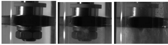
Fig. 1. The evolution of cavitation
