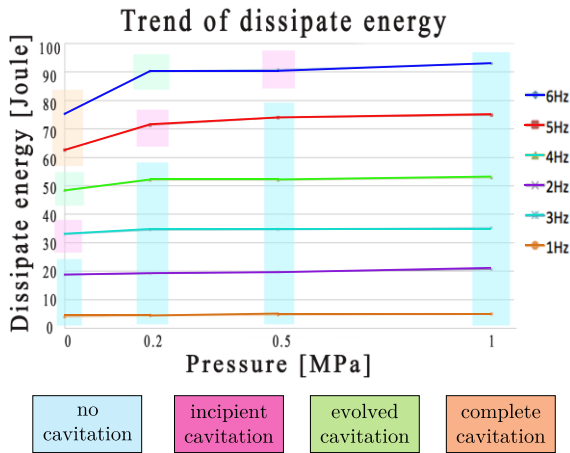
Fig. 14. Variation the performance of the shock absorber
