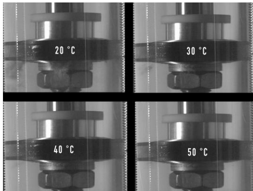
Fig. 11. Video acquisitions of piston, stressed 6 Hz, gas pressure 0.5 MPa, during the variation of the temperature
