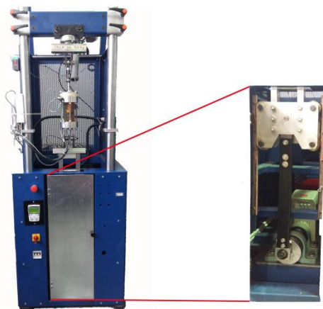
Fig. 2. The test bench and a detail of its road crank
