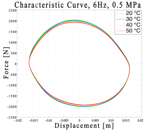
Fig. 12. Characteristic Curve, 6Hz, 0.5MPa, [20-30-40-50 °C]
