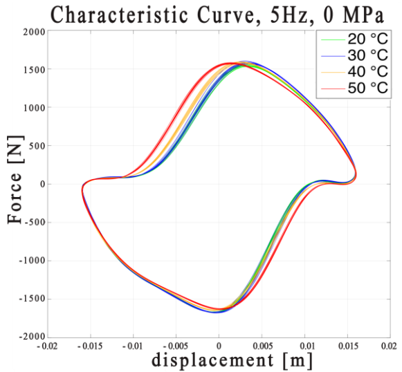
Fig. 13. Characteristic Curve, 5Hz, 0MPa, [20-30-40-50 °C]
