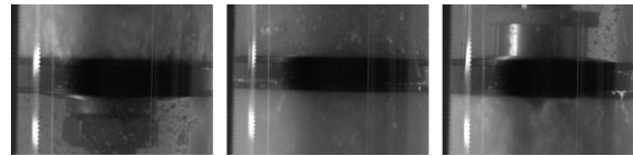
Fig. 8. Images acquisition of the test, 6Hz, 0MPa
