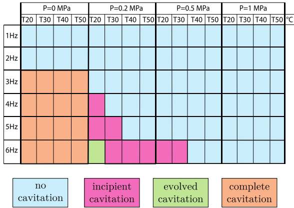
Fig. 10. Summary grid of an optical evaluation
