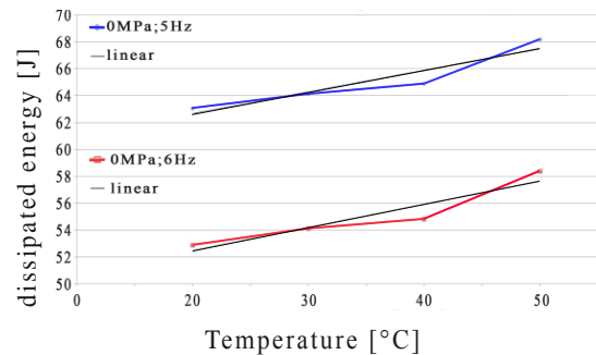
Fig. 16. Variation of the performance of the shock absorber. Full cavitation phase
