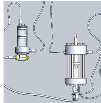
Fig. 3. Render of the transparent monotube shock absorber
