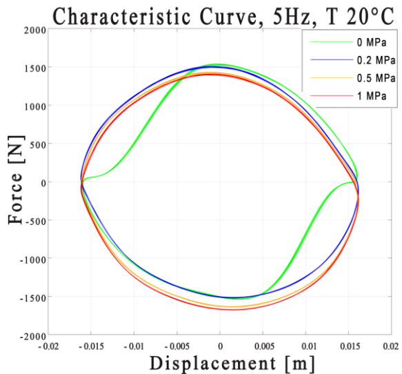
Fig. 9. Characteristic Curve, 5Hz, [0 - 0.2 - 0.5 - 1 MPa]
