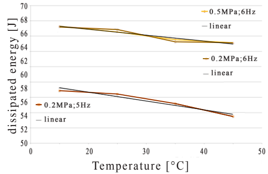
Fig. 15. variation of the performance of the shock absorber. Incipient or evolved cavitation
