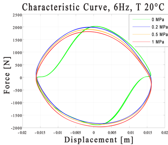
Fig. 5. Characteristic Curve, 6Hz, [0 - 0.2 - 0.5 - 1 MPa]
