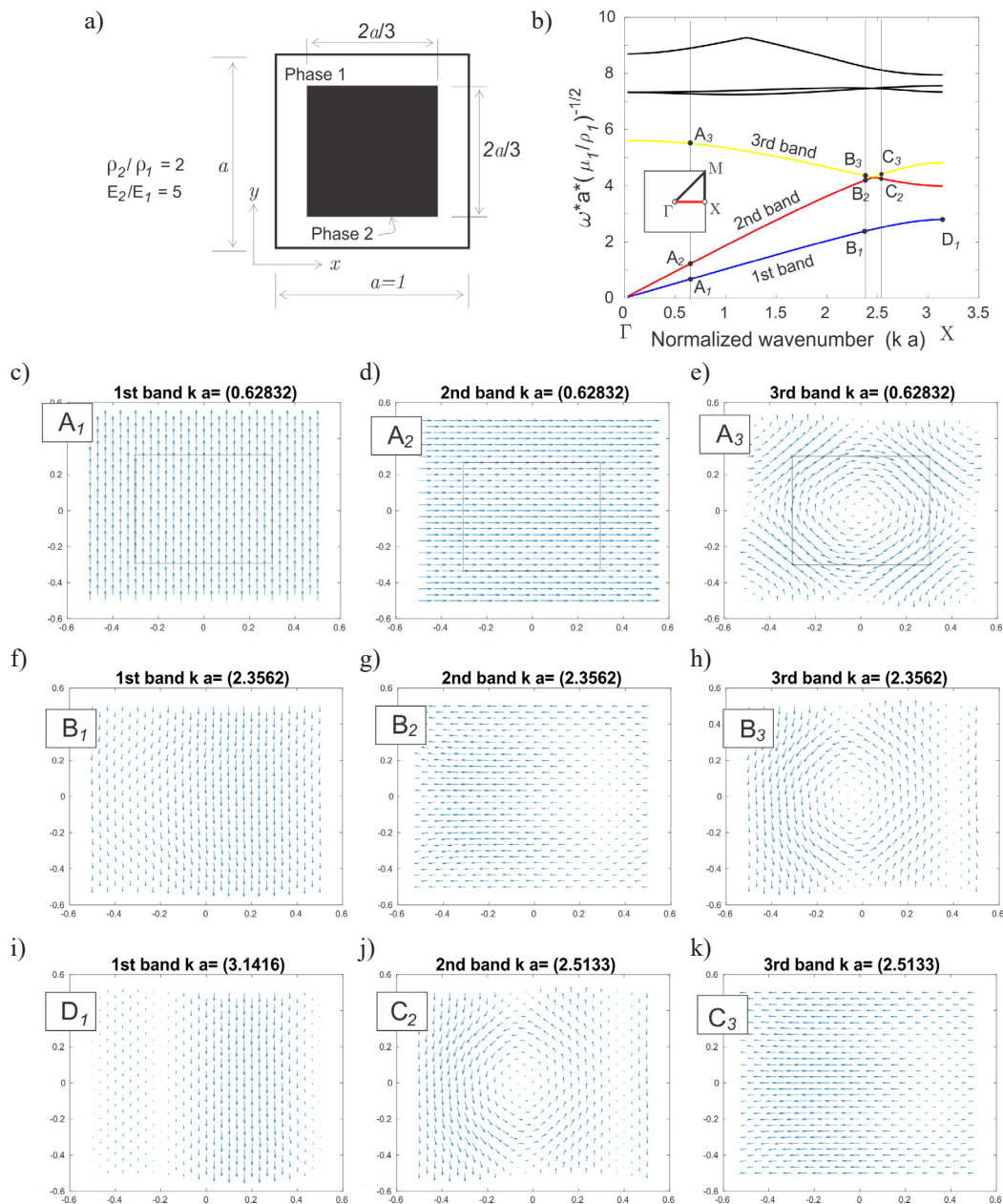
Fig. 5. Composite with square scatterers: a) microcell geometry; b) band structure for the six lower frequencies in the region \Gamma - X of the IFBZ; d–k) vector fields of the modes for the points A_1, A_2, \dots, D_1, C_2, C_3 , displayed in the band structure
