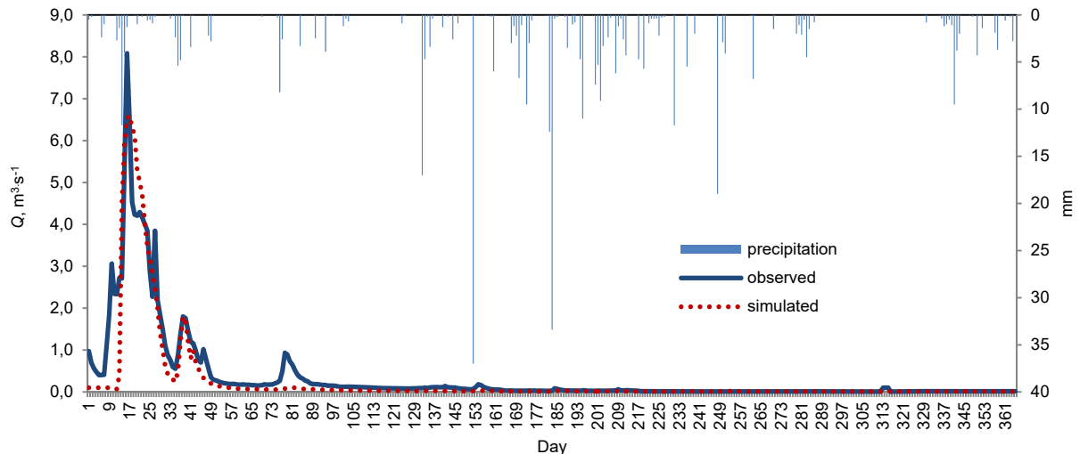
Fig. 6. Daily validation of discharge (2011); source: own study
