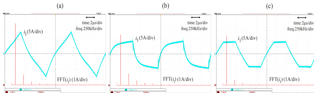
Fig. 5. Waveforms of the current and its spectrums in the high-voltage winding of the transformer in different load conditions: (a) short-circuit ( I_{1(\text{RMS})} = 8 \text{ A} ); (b) resistor ( I_{1(\text{RMS})} = 6.3 \text{ A} ); (c) bridge rectifier with an inductor in the DC circuit ( I_{1(\text{RMS})} = 6.7 \text{ A} )
