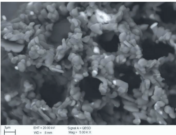
a) Fig. 3. Microstructure of ceramic preform fracture a) magnification 500x, b) magnification 5000x
