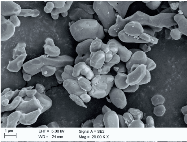
b) Fig. 2. Structure of Al 2 O 3 Alcoa CI 2500 powder: a) as delivered magnification 1000x, b) after the milling process, magnification 20,000x
