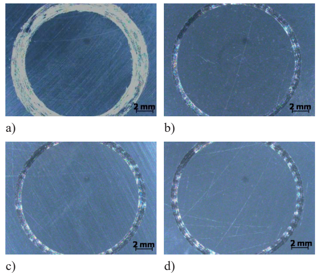
Fig. 4. Structure of wear traces: a) matrix EN AC - AlSi12, b) composite material with 20% content of ceramic phase, c) composite material with 24% content of ceramic phase, d) composite material with 33% content of ceramic phase
