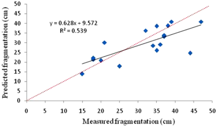
Fig. 5. Comparison between the real and predicted fragmentation for the Regression model
