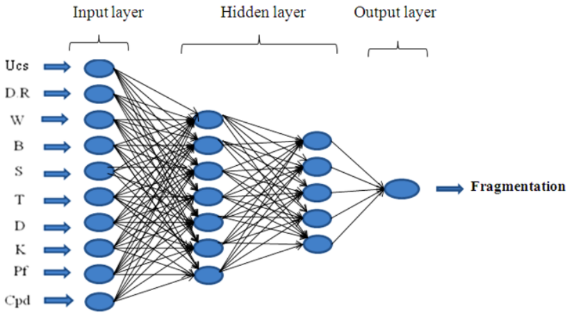
Fig. 3. The architecture of neural network model
