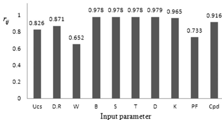
Fig. 7. The effect of input parameters on fragmentation
