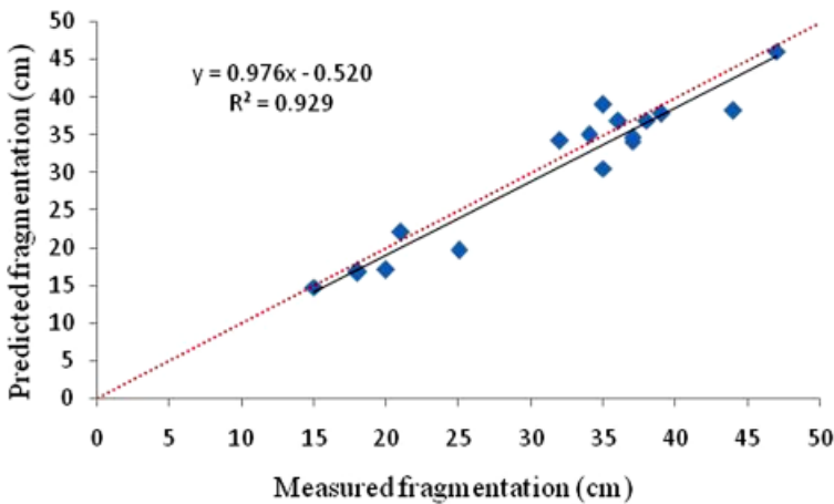
Fig. 4. Comparison between the measured and predicted fragmentation for the ANN model
