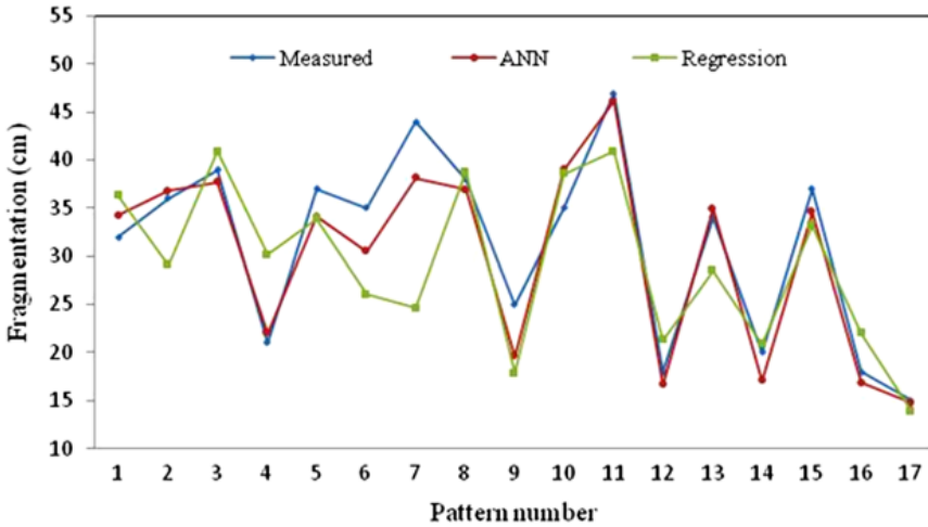
Fig. 6. Comparison of measured and predicted fragmentation
