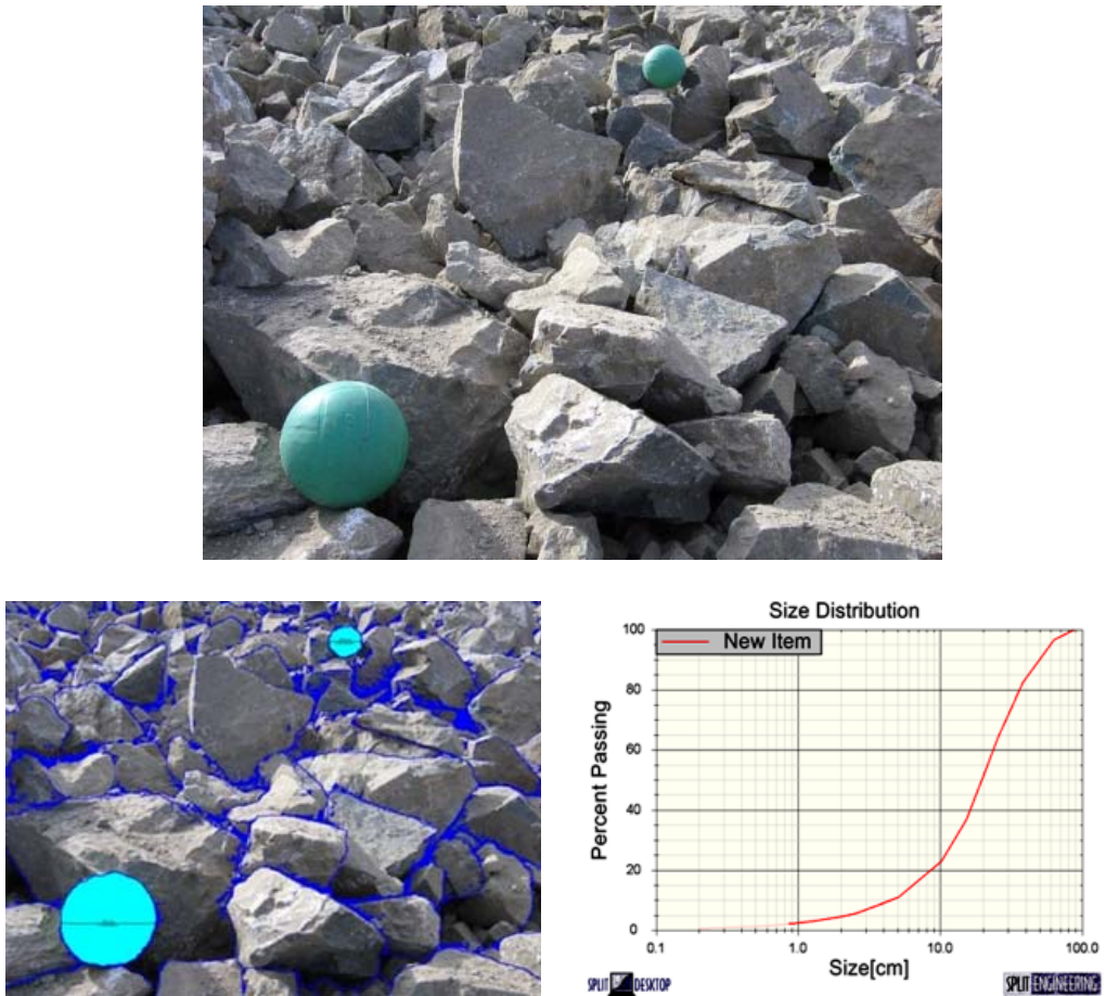
Fig. 1. Delineation of the muck pile image and its size distribution curve
