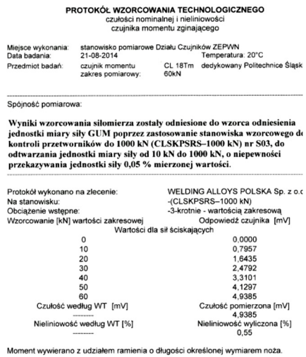
Fig. 10. Report from the technical calibration of the F_s force.
