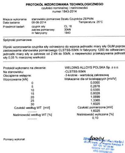
Fig. 12. Technological calibration protocol of the F_d force
