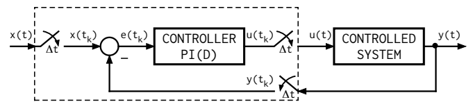
Fig. 3. Discretized automatic control system.
