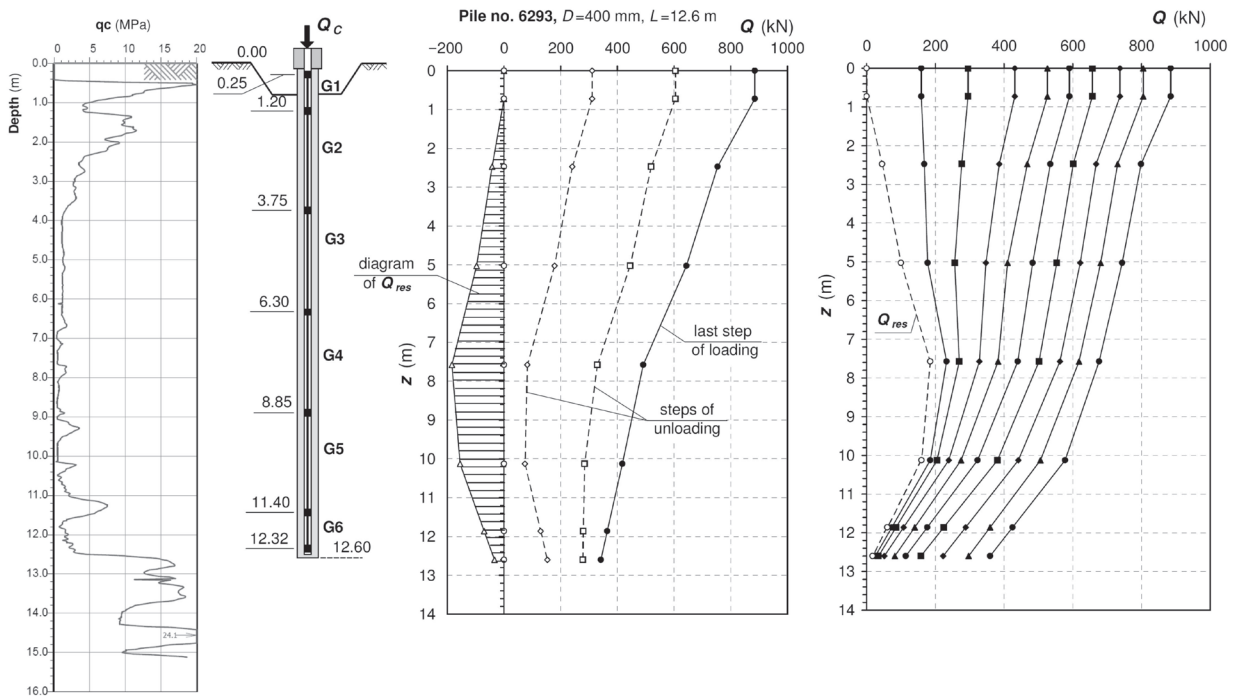
Figure 8: Pile no. 6293: (a) determination of the residual force in the pile shaft and (b) its inclusion in the distribution of the axial force along the pile in successive load steps.
