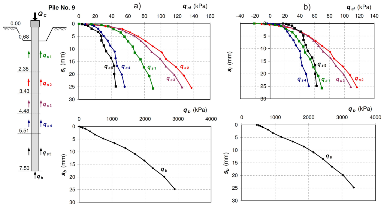
Figure 18: Pile no. 9, comparison of q_s and q_b unit soil resistances around the pile for the cases: a) without taking into account the residual force and b) taking into account the residual force.
