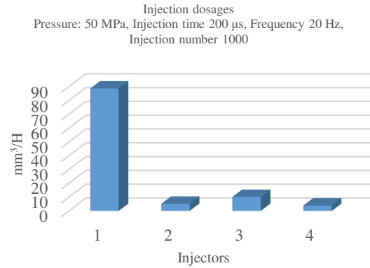
Fig. 13. Injector work test results. Pressure 50 MPa, injection time 200 \mu s
