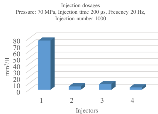
Fig. 15. Injector work test results. Pressure 70 MPa, injection time 200 \mu s
