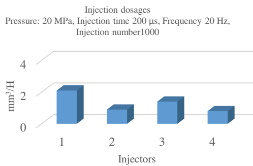
Fig. 10. Injector work test results. Pressure 20 MPa, injection time 200 \mu s
