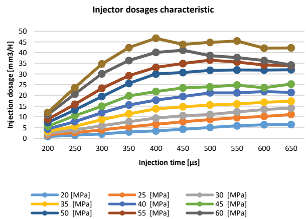
Fig. 21. Faulty injector work characteristic
