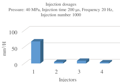
Fig. 12. Injector work test results. Pressure 40 MPa, injection time 200 \mu s
