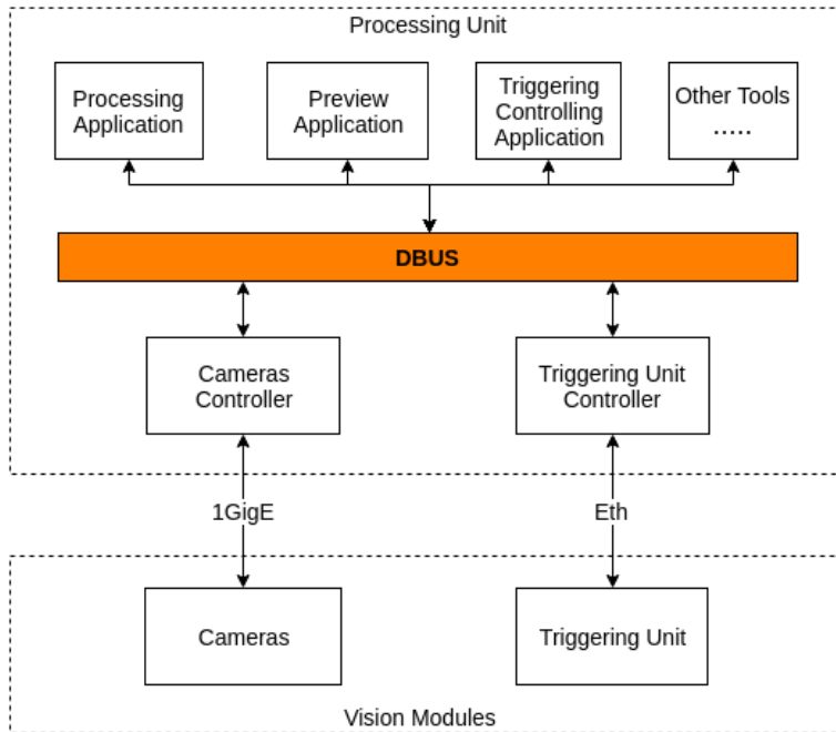
Figure 2. Software architecture.
