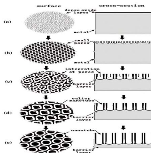
Figure 1. The evolution of straight nanotubes at a constant anodization voltage
