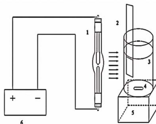
Figure 2. Diagram of the equipment for photocatalytic oxidation (1. Xenon lamp; 2. Working electrode; 3. Quartz reactor; 4. Stirrer; 5. Magnetic stirrer and 6. Power supply)
