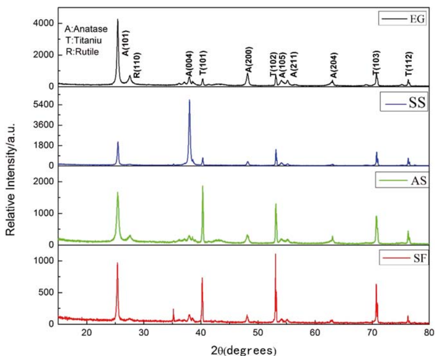
Figure 4. XRD patterns of the fabricated TiO 2 NTAs. (1) EG-type, (2) SS-type, (3) AS-type and (4) SF-type
