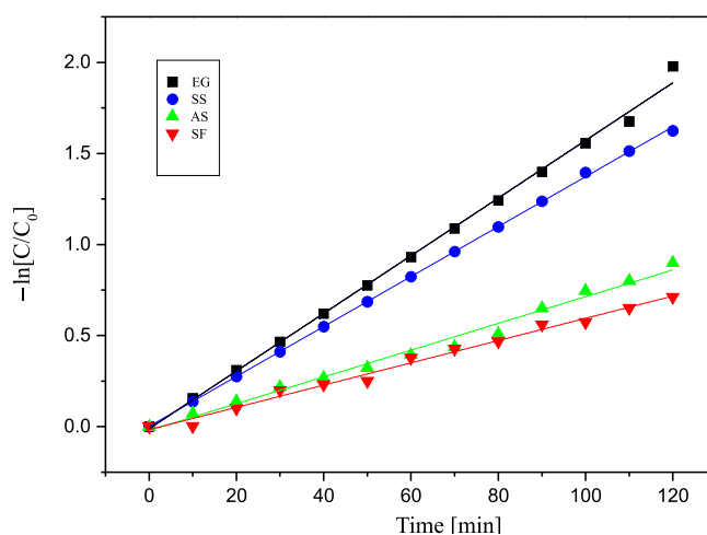
Figure 7. PC evolution curves of RhB solution on as-prepared bare TiO 2 NTAs photoelectrodes under 120 min of xenon light illumination
