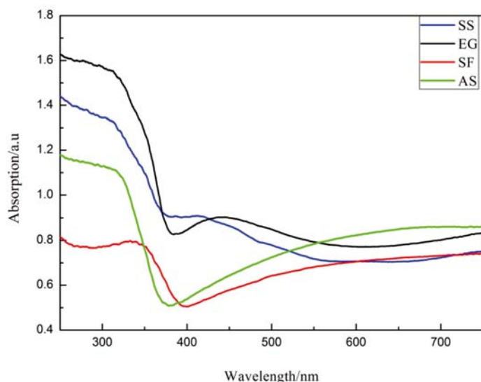
Figure 5. UV-Visible light absorption DRS patterns
