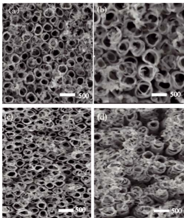
Figure 3. SEM analysis (a) Nanotubes EG type, (b) Nanotubes SS type, (c) Nanotubes AS type, and (d) Nanotubes SF type
