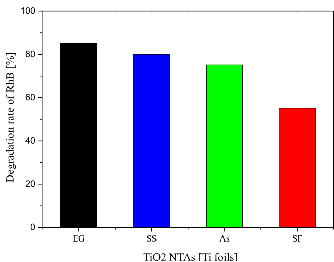
Figure 9. The photocatalytic degradation efficiency of the fabricated bare TiO 2 NTAs in different electrolyte mixtures
