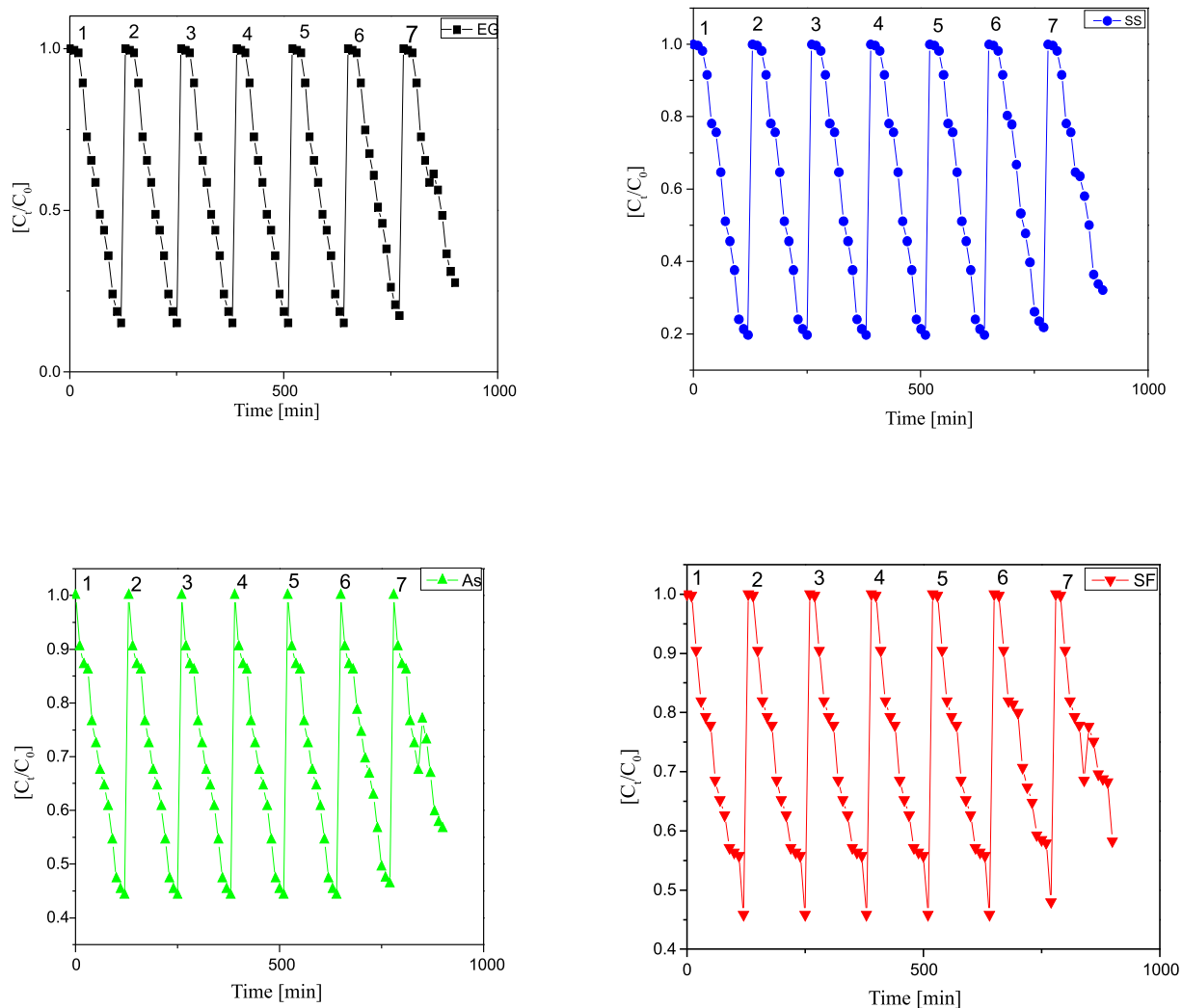
Figure 8. Photocatalyst stability test of as-prepared bare TiO 2 NTAs photoelectrodes (1) EG-type, (2) SS-type, (3) AS-type and (4) SF-type
