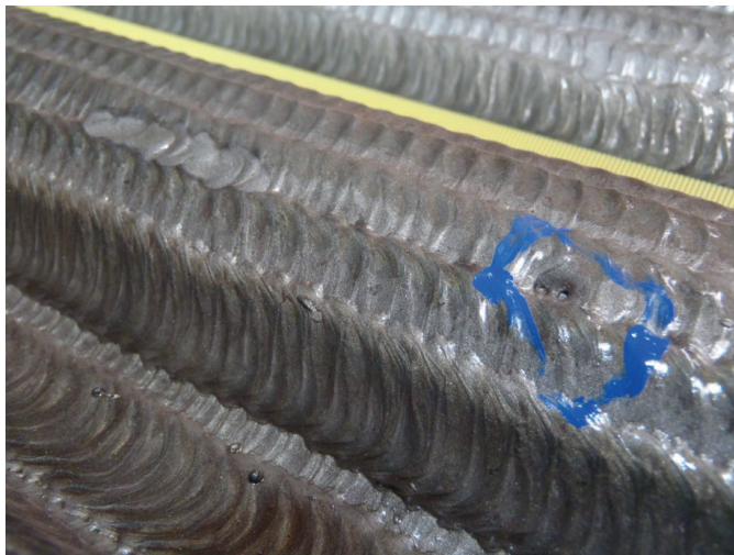
Fig. 1. Piping in the surfacing weld Source: own collections
