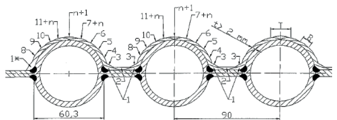
Fig. 4. The WPS sketch showing the way of making beads of the surfacing weld on the sheet pile wall in the scale 90 mm (Ø 60,3 mm pipe) Source: own study
