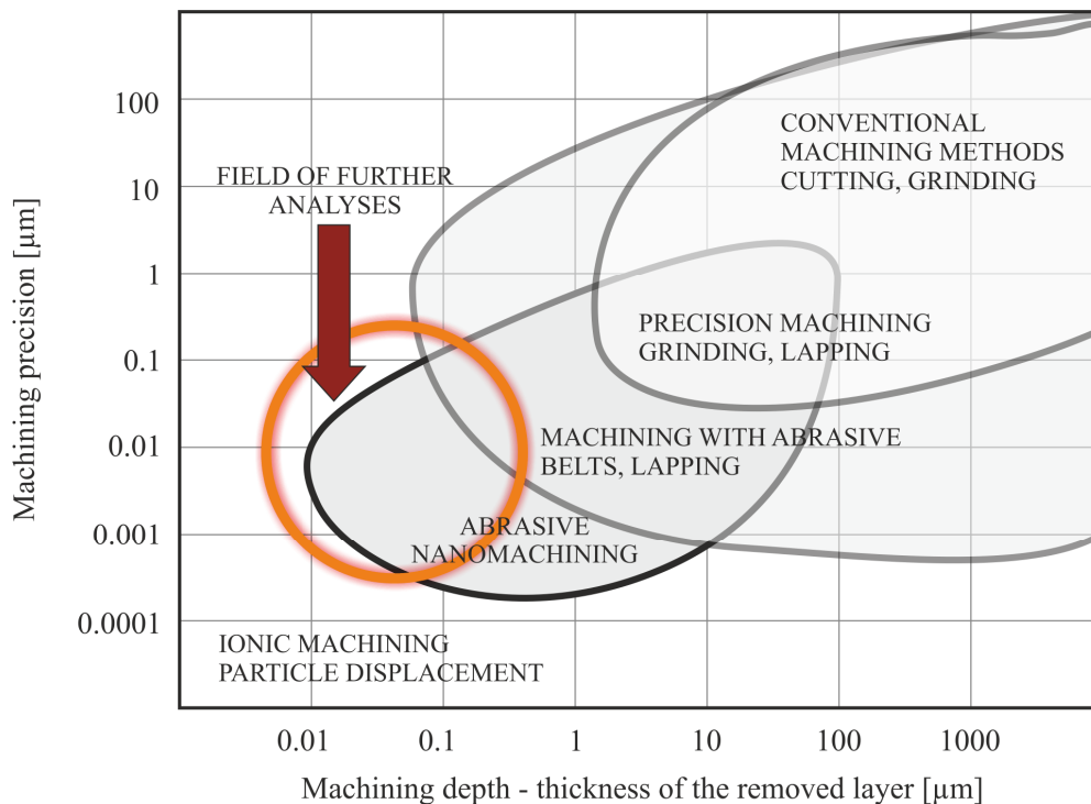
Fig. 1. Area of abrasive nanomachining
