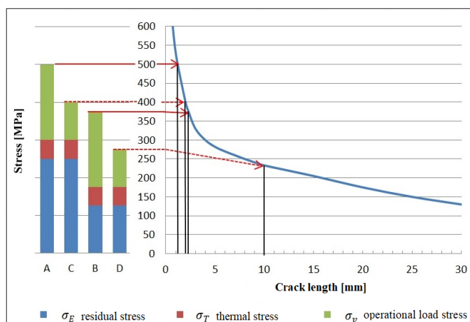
Fig. 1. Dependence of critical crack length on tensile stress [1]
