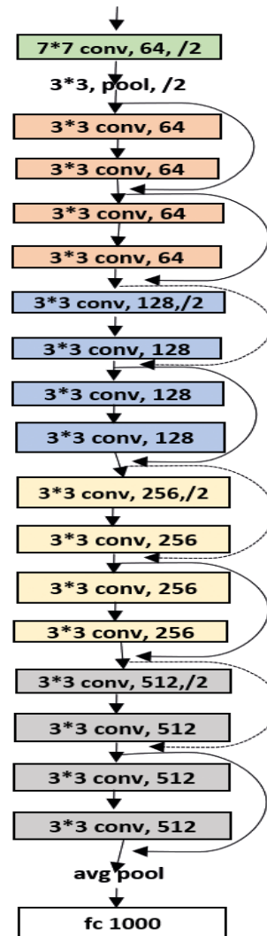
Figure 6. Resnet18 Architecture
