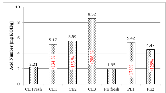
Fig. 5. Changes in the acid number of the tested engine oil samples
