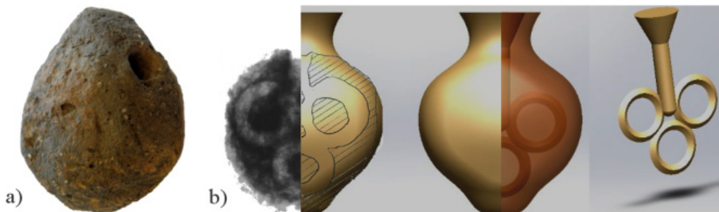
Fig. 4. Casting mold (a) [27]; graphic documentation based on radioscopic image: visualization of casts connected by gating system comparison with X-ray image and visualization of casting mold (b)
