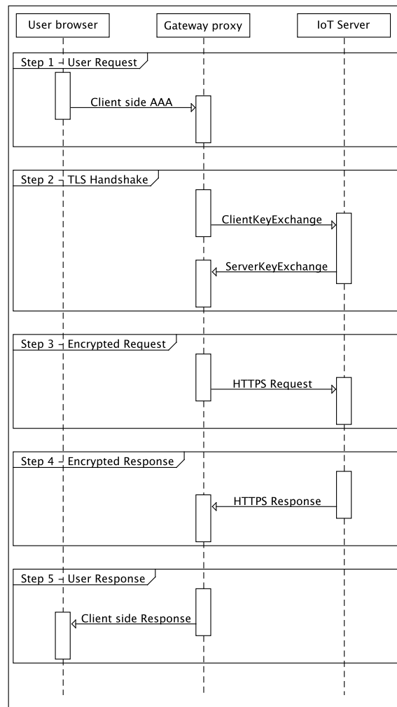
Figure 5 Standard communication process between Gateway and IoT Device.
