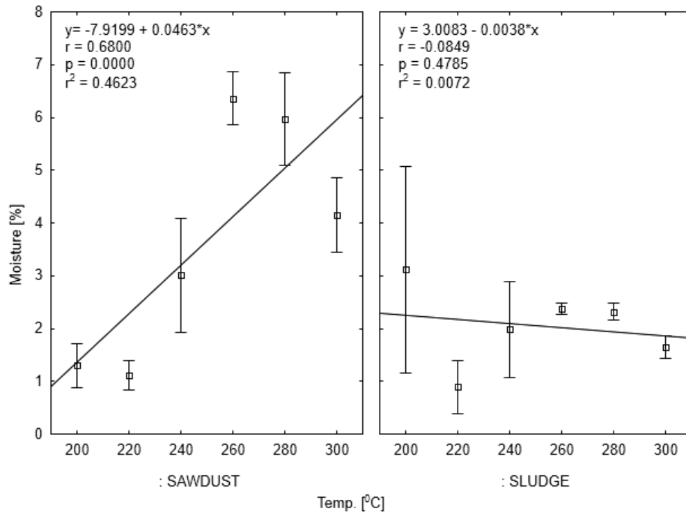
Fig. 2. Correlation between moisture biocarbons [%] and process temperature
