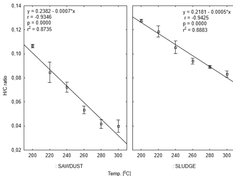
Fig. 9. Correlation between H/C ratio of biocarbons and process temperature
