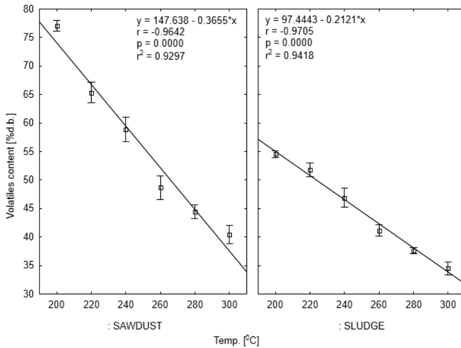
Fig. 6. Correlation between volatiles content [% d.b.] in biocarbons and process temperature
