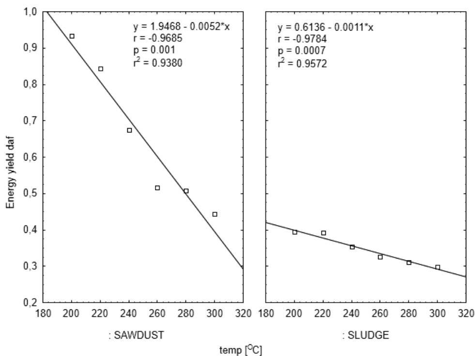
Fig. 5. Correlation between energy residue [%] in biocarbons and process temperature
