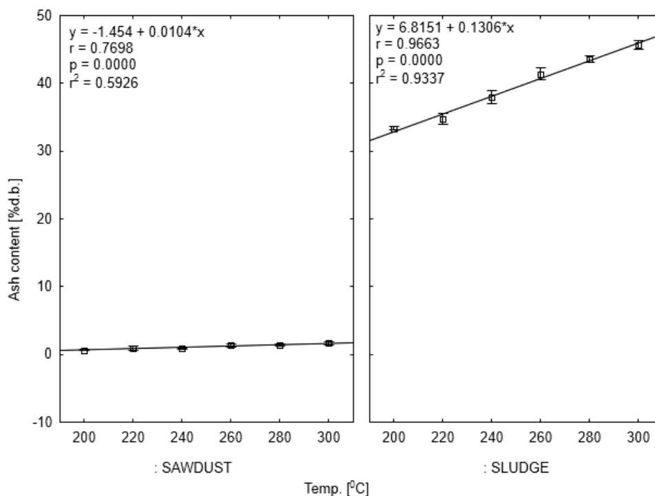
Fig. 7. Correlation between ash content [% d.b.] in biocarbons and process temperature
