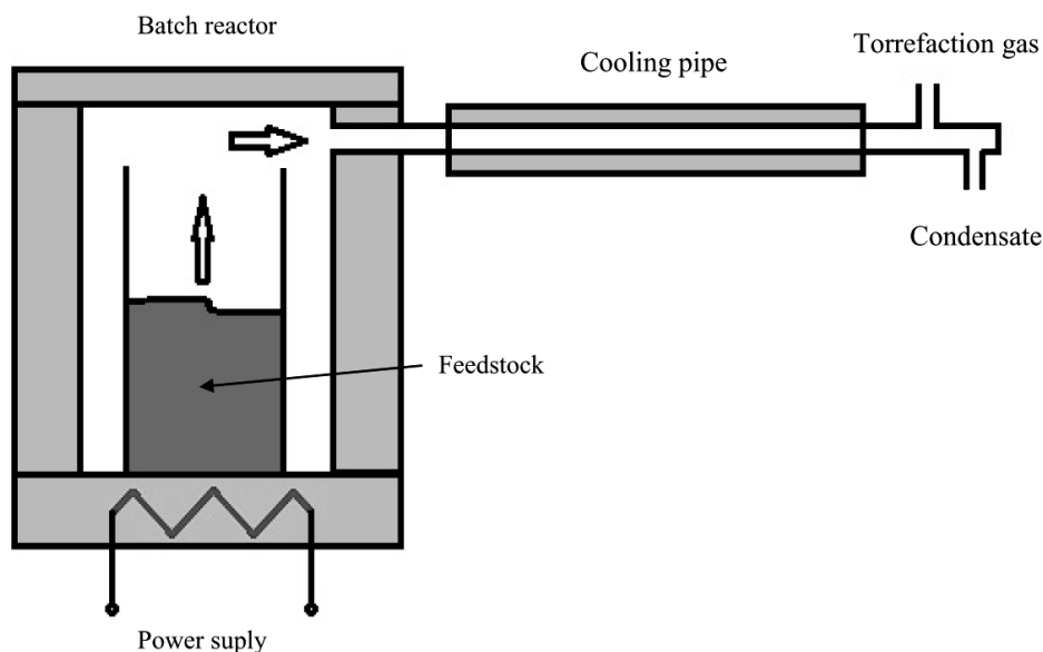
Fig. 1. Design of torrefaction batch reactor
