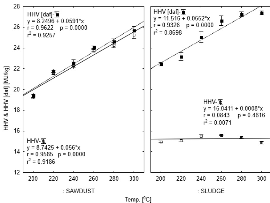
Fig. 4. Correlation between HHV and HHV [daf] [MJ/kg d.b.] of biocarbons and process temperature
