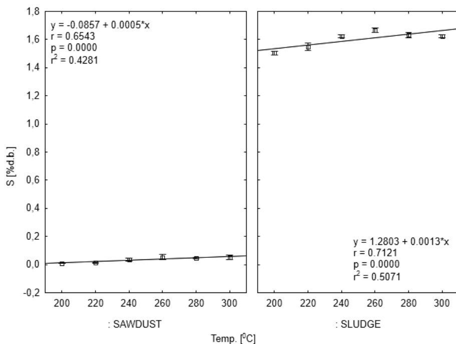
Fig. 8. Correlation between sulfur content [% d.b.] in biocarbons and process temperature
